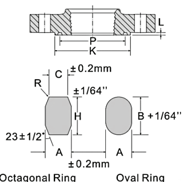
Octagonal Ring
