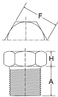
Plug / Bushing | ASME B16.11
