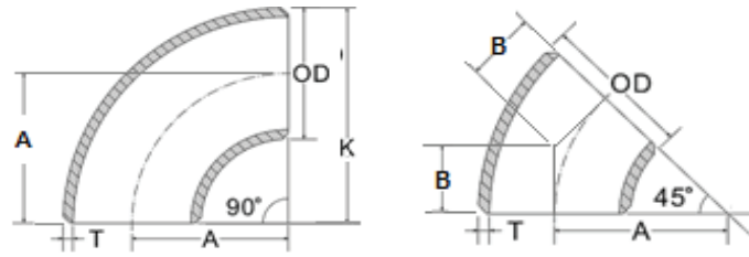
Elbow | Short Radius | ASME/ANSI B16.9
