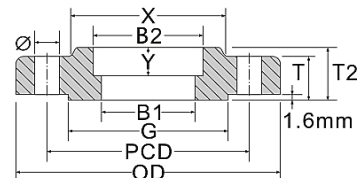
Socket Welding
