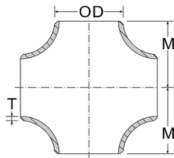
Equal Crosses | ASME/ANSI B16.9
