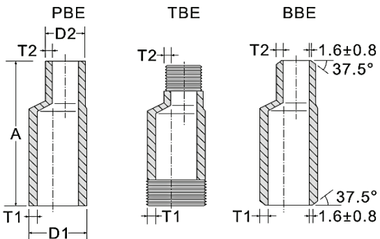
Eccentric
