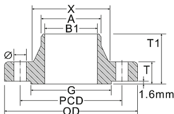
Welding Neck
