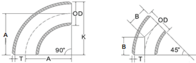
Elbow | Long Radius | ASME/ANSI B16.9
