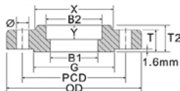
Socket Welding
