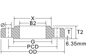
Slip-on
