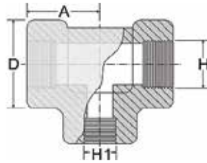
Reducing Tee
