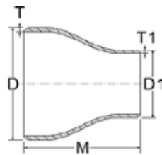
Concentric and Eccentric Reducers | ASME/ANSI B16.9
