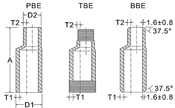
Eccentric
