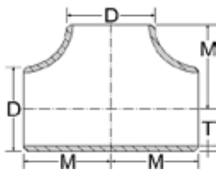
Equal Tee
