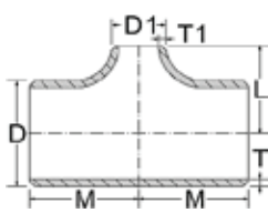
Reducing Tee
