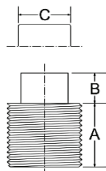
Plug / Bushing | ASME B16.11
