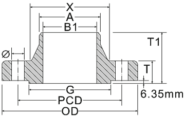
Welding Neck
