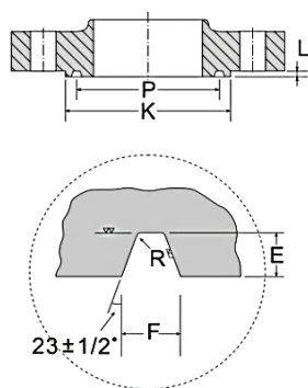
Octagonal Ring
