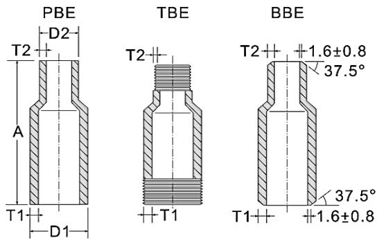
Concentric
