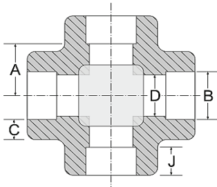
Cross
