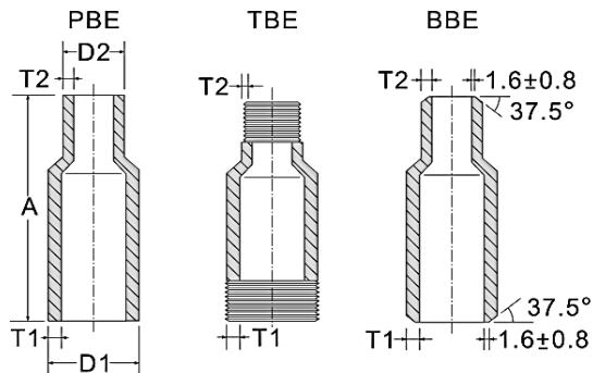
Swaged Nipple | Plain | MSS SP 95
