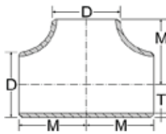
Equal and Reducing Tees | ASME/ANSI B16.9
