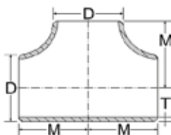
Equal and Reducing Tees | ASME/ANSI B16.9
