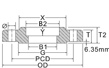
Socket Welding
