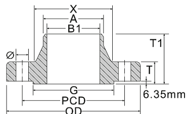
Welding Neck
