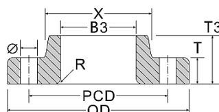
Lap Joint
