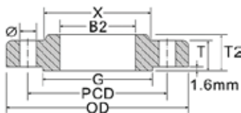
Slip-on
