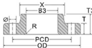
Lap Joint
