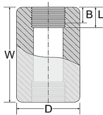
Coupling
