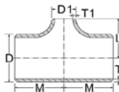
Reducing Tee
