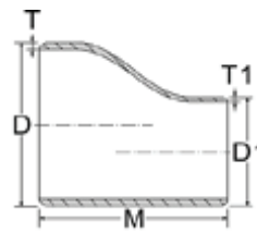
Concentric and Eccentric Reducers | ASME/ANSI B16.9
