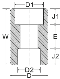
Reducing Coupling
